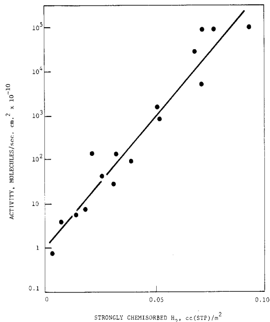
Figure 5. Correlation of ethane hydrogenolysis activity and amount of strongly chemisorbed hydrogen for ruthenium-copper catalysts. The ethane hydrogenolysis activities are rates at 245 °C and ethane and hydrogen pressures of 0.030 and 0.20 atm, respectively. The amount of strongly chemisorbed hydrogen at room temperature was determined as in Figures 1 and 2. 18
